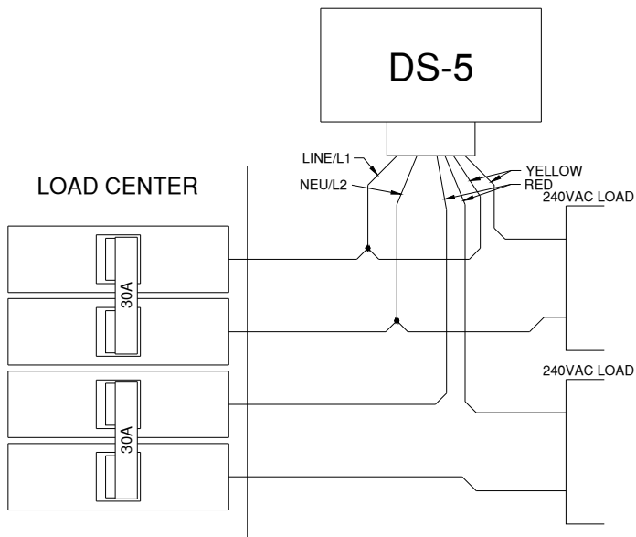
240VAC In, Dual 240VAC Loads (Strap DS-5 for 240VAC Power)
