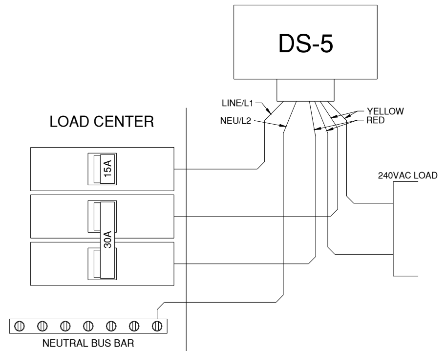
120VAC In, 240VAC Load, Heat Cable or Similar (Strap DS-5 for 120VAC Power)
