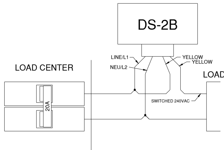
240VAC In, 240VAC Load, Heat Cable or Similar (Strap DS-2B for 240VAC Power)
