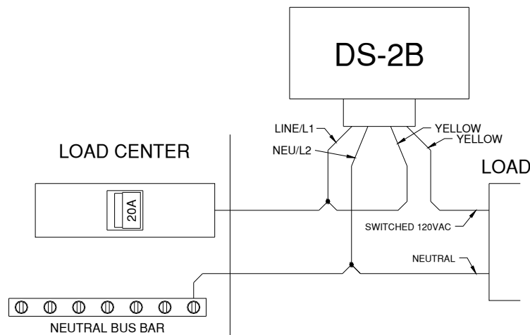
120VAC In, 120VAC Load, Heat Cable or Similar (Strap DS-2B for 120VAC Power)
