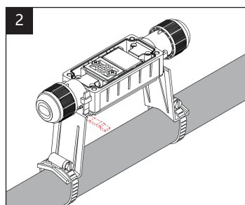
2. Align and insert the four clips of the mounting bracket with the four holes of the quick connector. Note: installation direction of quick connector
