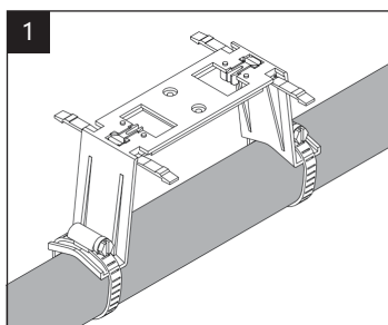
1. Fix the bracket on the pipe line with steel belt Note: do not install the connector at the place where water is completely invaded
