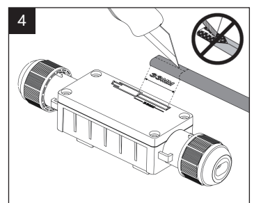
4. Cut the outerjacket from the middle at 33mm away from the cutting section with an utility knife, and remove the outerjacket.
