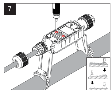
7. Tighten the two screws on the cover plate of the connector alternately to ensure the screw is locked. Note: there is a fire hazard. Loose screws may cause heating and sparking. Please ensure that the screws are locked.
