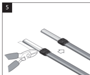
5.2 Heating cable which have aluminum foil layer Pull exposed braid back and tidy it., and cut the aluminum foil layer.
