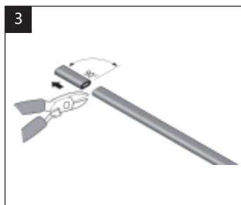
3. Cut off the cable according to the length required for installation. Note: the cable cutting section shall be flat and tidy
