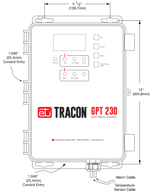
FIGURE 2. Mounting Dimensions
