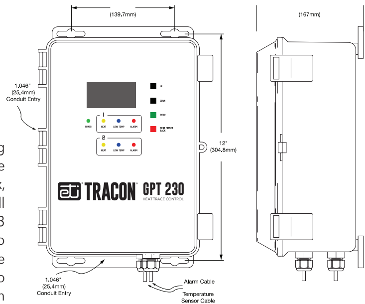
FIGURE 2. Mounting dimensions.
