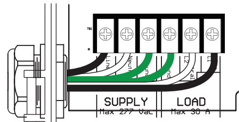
FIGURE 3. Contractor connections.
