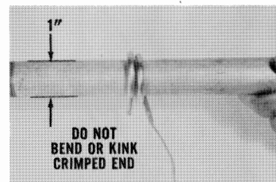
Figure 3 (Sensing Bulb)
