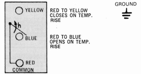
Figure 5 — Terminal arrangement
